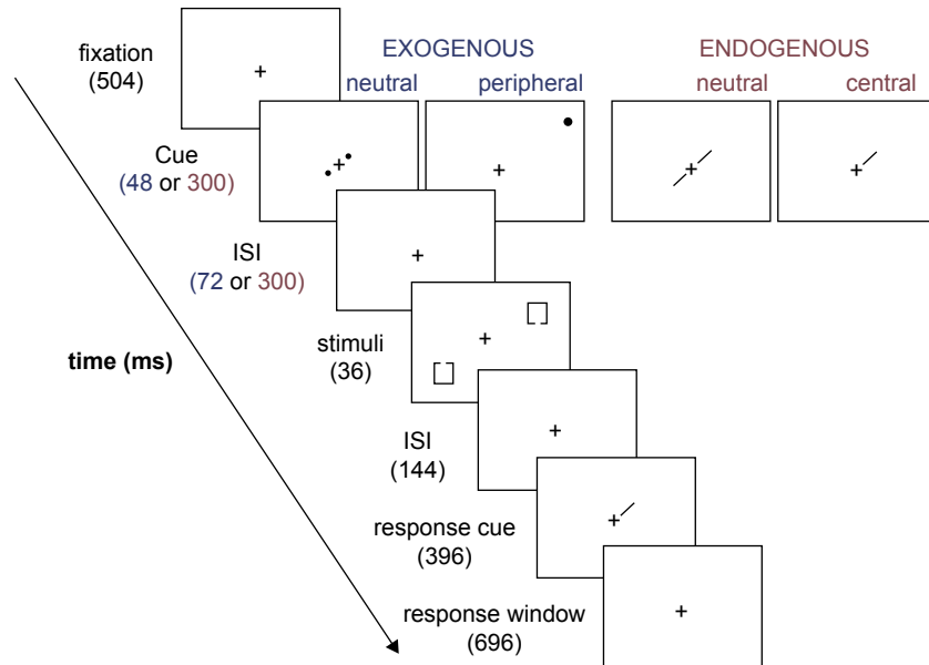
Fig. 4. Trial sequence. The trial sequence was identical for the exogenous and endogenous attention conditions except for the spatiotemporal characteristics of the peripheral and central cues. Adapted from Montagna et al. (2009).
