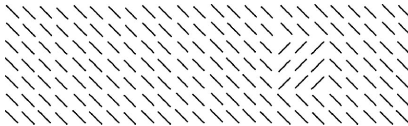
Fig. 7. Example of the texture stimuli used in Yeshurun and Carrasco (1998).
