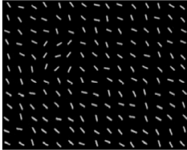
Fig. 14. An example of the heterogeneous textures used in Yeshurun et al. (2008).
