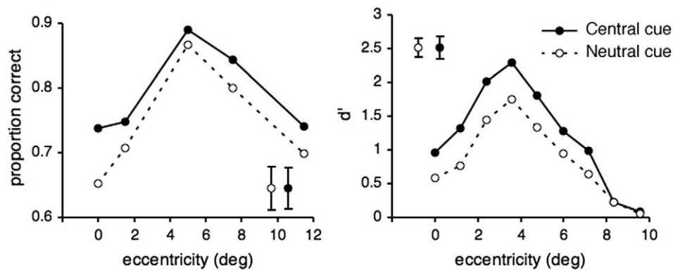
Fig. 15. Observers' performance as a function of cue condition and target eccentricity, for texture stimuli with homogeneous (left panel; see Fig. 7) or heterogeneous (right panel; see Fig. 14) background. Adapted from Yeshurun et al. (2008).
