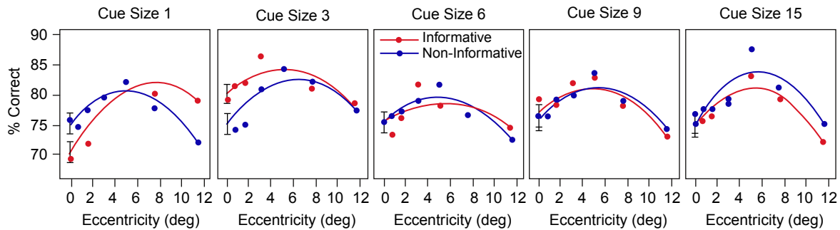
Fig. 13. Observers' performance as a function of cue size and target eccentricity. "Informative" refers to the trials in which the cue carried some information regarding the target location (the larger the cue the less precise this information is). "Noninformative" refers to the trials in which the cue carried no information regarding the target location (the largest cue). The number of cue size indicates the number of texture columns encompassed by the cue frame. Adapted from Yeshurun and Carrasco (2008).
