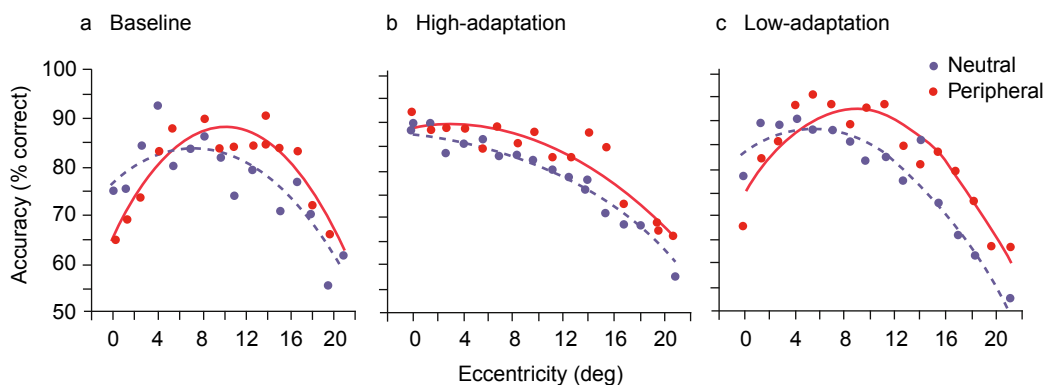
Fig. 11. Observers' performance as a function of cue type and target eccentricity. (a) Baseline, (b) high-spatial-frequency adaptation grating, and (c) low-spatial-frequency adaptation grating. Adapted from Carrasco et al. (2006).
