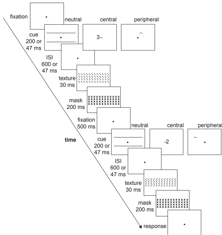
Fig. 1. Schema of the frame sequence in a typical trial with a central (sustained attention) or peripheral (transient attention) cue in a 2IFC texture segmentation task. The participants had to indicate which of the two intervals included a texture target whose orientation was orthogonal to that of the texture background. In this example the target is present in the second interval. The peripheral cue is a small horizontal bar appearing above the target location, and the central cue is composed of a digit indicating the eccentricity at which the target may appear and a line indicating the hemifield in which the target may appear. Adapted from Yeshurun et al. (2008).
