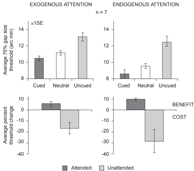
Fig. 5. Average gap-size thresholds (75% localization accuracy) for both exogenous (upper-left panel) and endogenous (upper-right panel) attention for the cued, neutral, and uncued conditions. The lower panels depict the average percent change in acuity thresholds at cued and uncued locations as compared to the neutral condition for exogenous (left) and endogenous (right) attention. Values below zero indicate a cost in acuity, whereas values above zero indicate a benefit. Error bars show \pm 1 SE. Adapted from Montagna et al. (2009).
