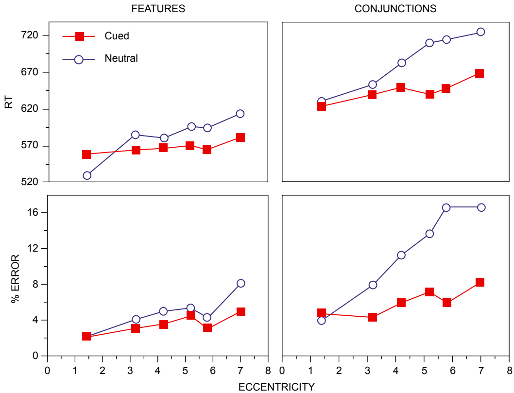
Fig. 6. RT and error rate for feature search (left panel — a search for a red vertical line appearing among red tilted lines) and conjunction search (right panel — a search for a red vertical line appearing among red tilted and blue vertical lines). Adapted from Carrasco and Yeshurun (1998).
