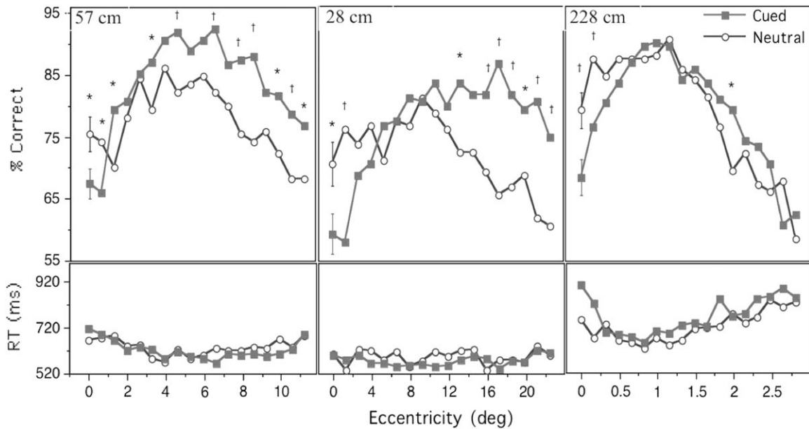
Fig. 8. Observers' performance as a function of target eccentricity and cueing condition for the three viewing distances. Because viewing distance varied, the eccentricity values (abscissa) differ in the three panels. Adapted from Yeshurun and Carrasco (1998).
