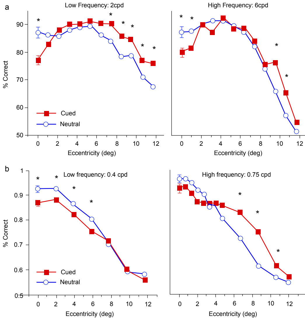
Fig. 10. Performance with first-order (a) and second-order (b) textures of low (left) or high (right) frequency as a function of cueing condition and target eccentricity. Adapted from Yeshurun and Carrasco (2000).
