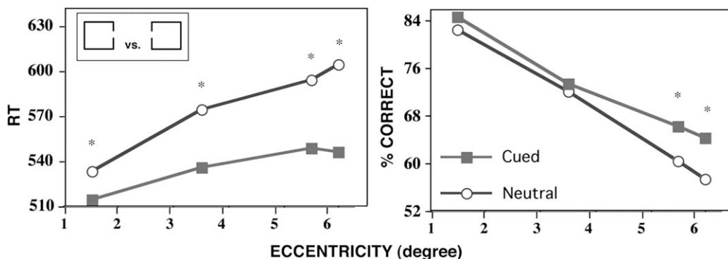
Fig. 2. RT (left panel) and accuracy (right panel) for detection of a gap in a Landolt-square (inset). Adapted from Yeshurun and Carrasco (1999).
