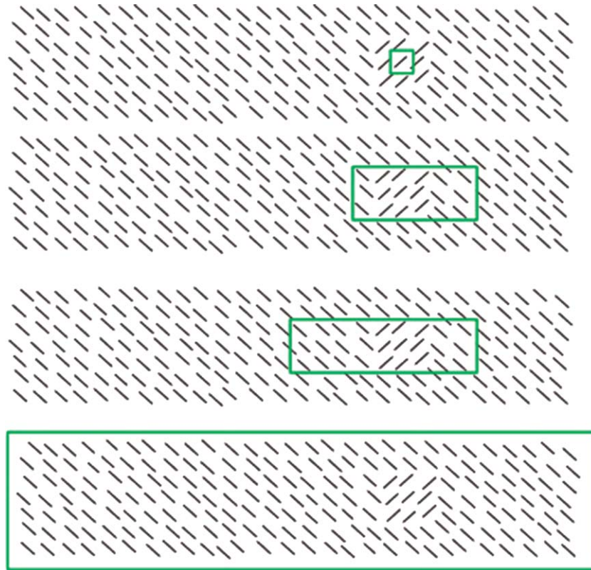
Fig. 12. An example of cues of different sizes and the textures used in Yeshurun and Carrasco (2008). The largest cue (bottom) was similar to the neutral cue employed previously (e.g., Yeshurun and Carrasco, 1998), and since it carried no information regarding the target location this cue served as the baseline to which performance with smaller cues was compared.
