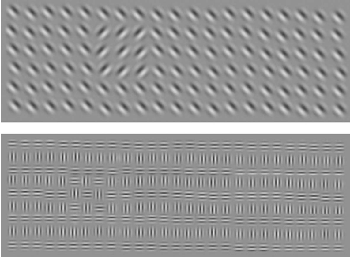
Fig. 9. An example of the first-order (top) and second-order (bottom) textures used in Yeshurun and Carrasco (2000).
